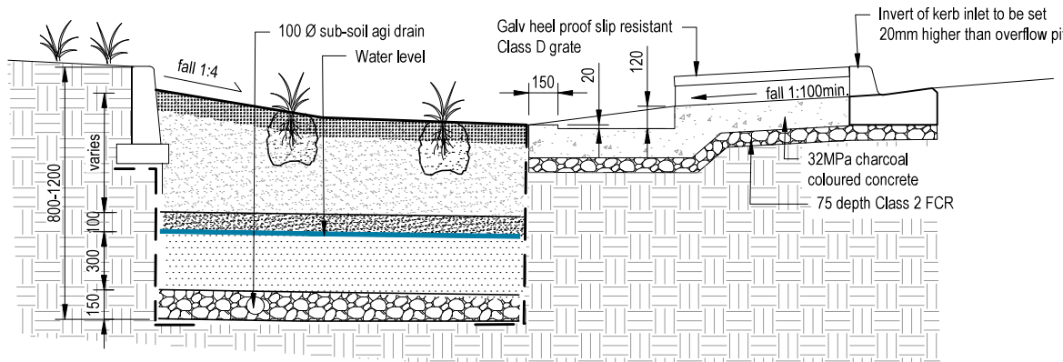
B SECTION
