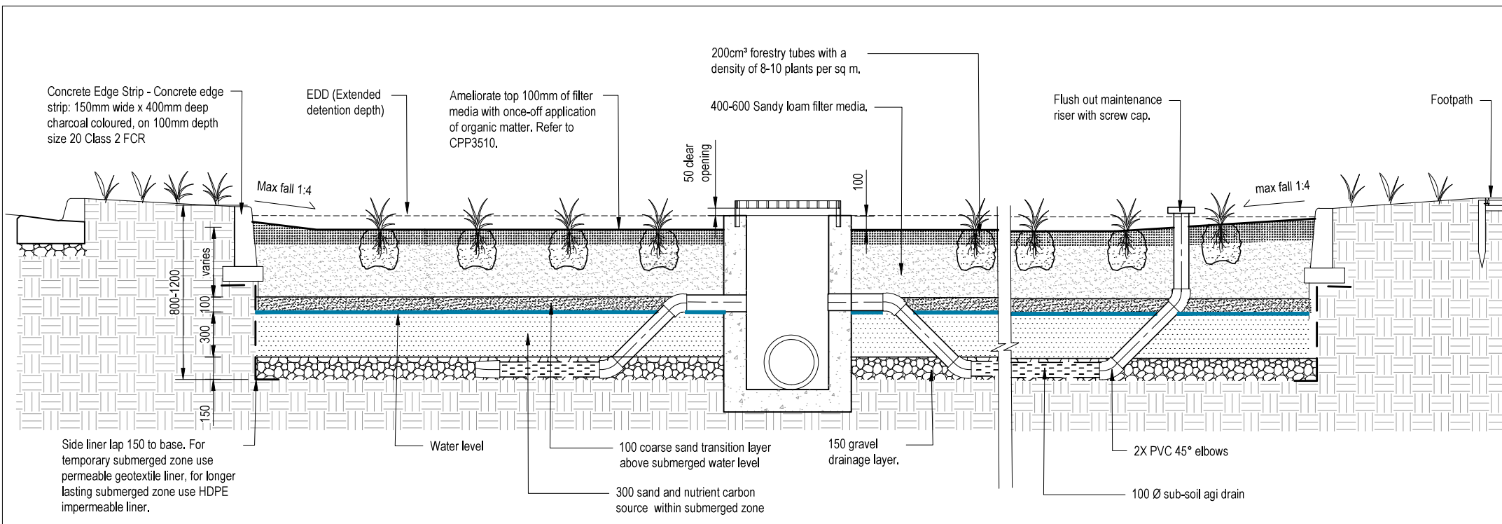
A SECTION
