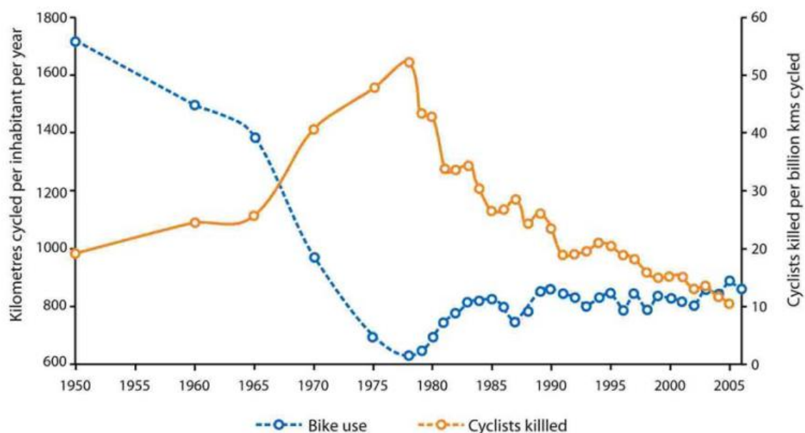
Figure 4: Annual kilometres cycled per inhabitant in the Netherlands and cycling fatality rates, 1950–2005
