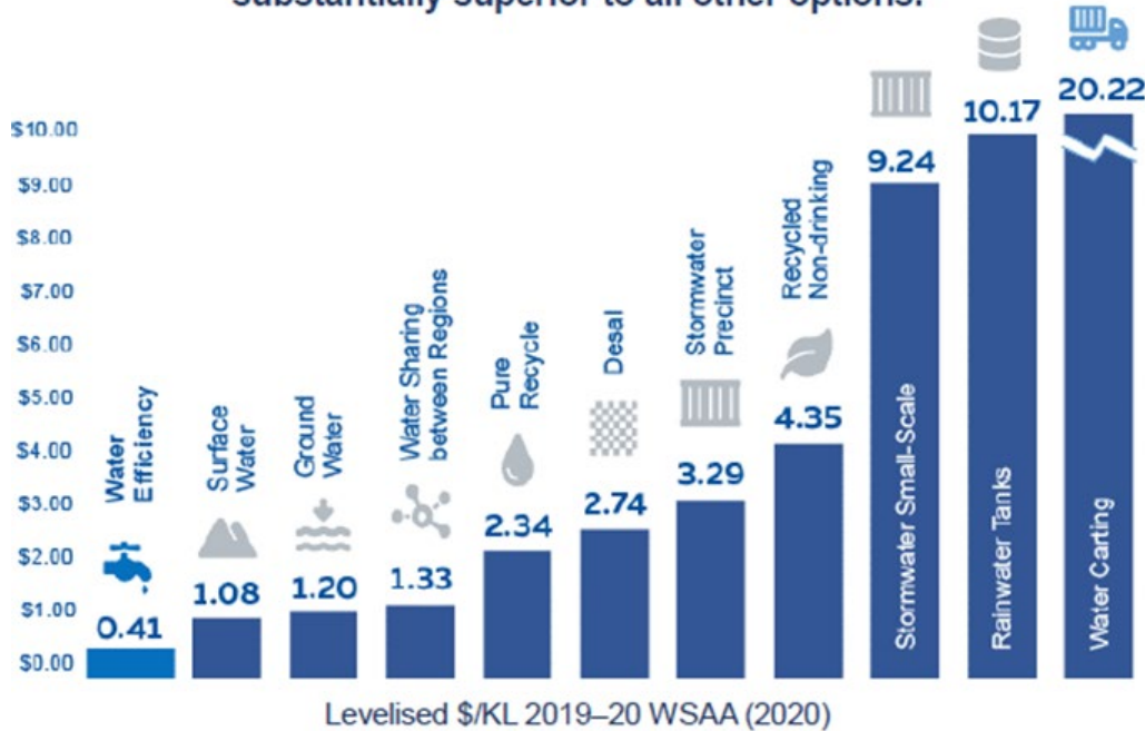
Figure 23: Levelised cost of various water supply and demand management options 47
