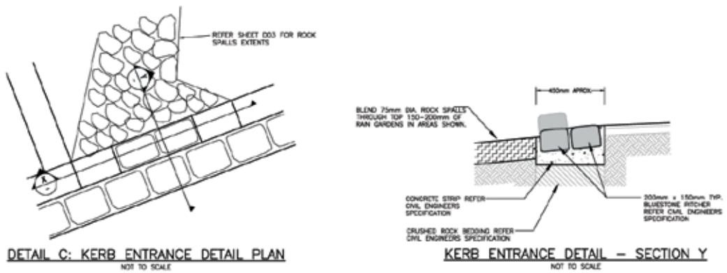
Figure 35. Kerb entrance and section detail
